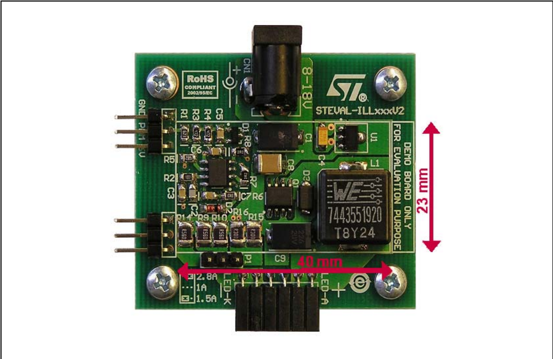
Figure 6. Reference design detail
