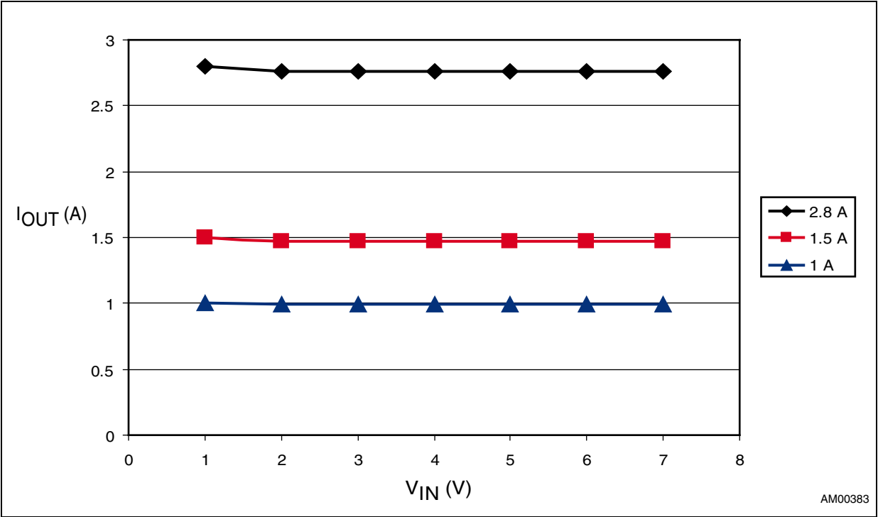
Figure 11. Variation in output current vs. input voltage (1 LED load)
